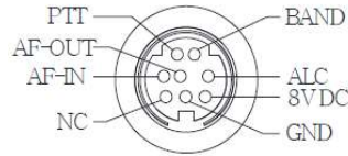
Rear ACC socket
